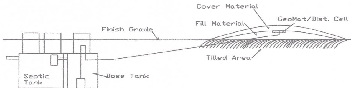
Figure 1: Cross section of a GeoMat mound system
